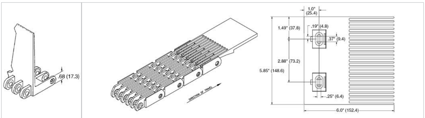
Flights Standard flights are available in 1", 2", 3" and 4" heights Fluid-Flo transfer plate Part number TP-FF6
